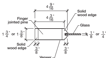
SIDERAIL
