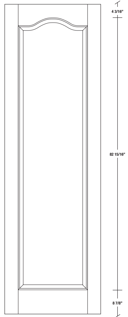
2010S / 2910S
