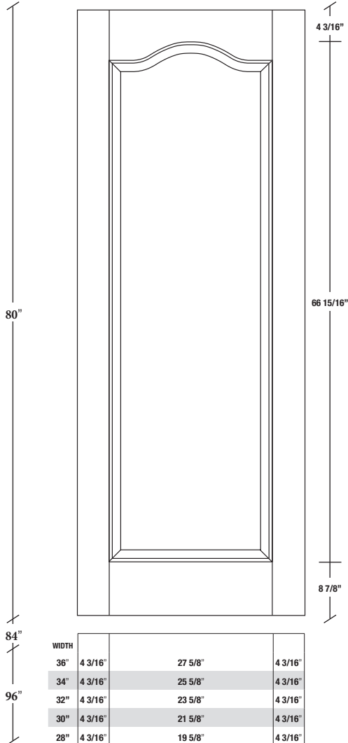
2010S / 2910S
