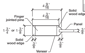
SIDERAIL FLAT PANEL #29XX
