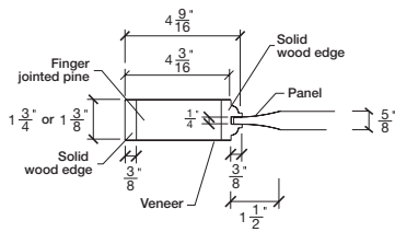
SIDERAIL RAISED PANEL #30XX
