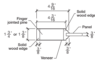
SIDERAIL FLAT PANEL #39XX
