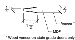
5" PANEL * Wood veneer on stain grade doors only
