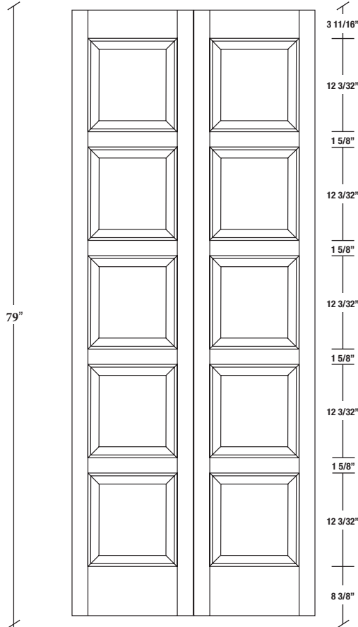
205LP / 295LP
