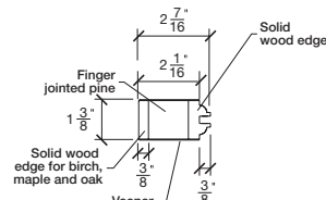
1 \frac{3}{8} " SIDERAIL
